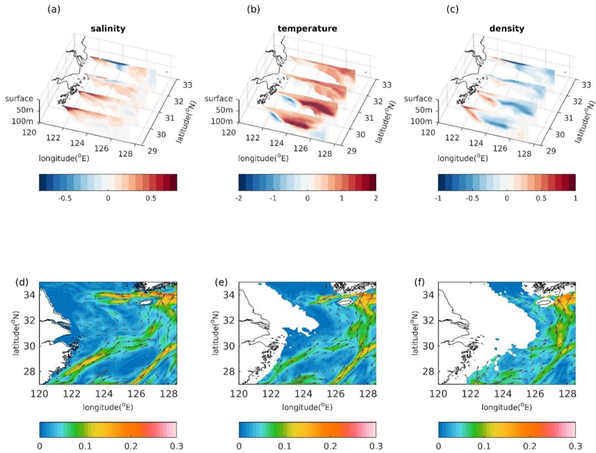
Fig. 14. The composites of Type I (a) salinity (b) temperature (c) density anomaly during July. (d)–(f) anomalous circulation (m/s) at 10 m, 40 m, and 70 m during July, respectively.
