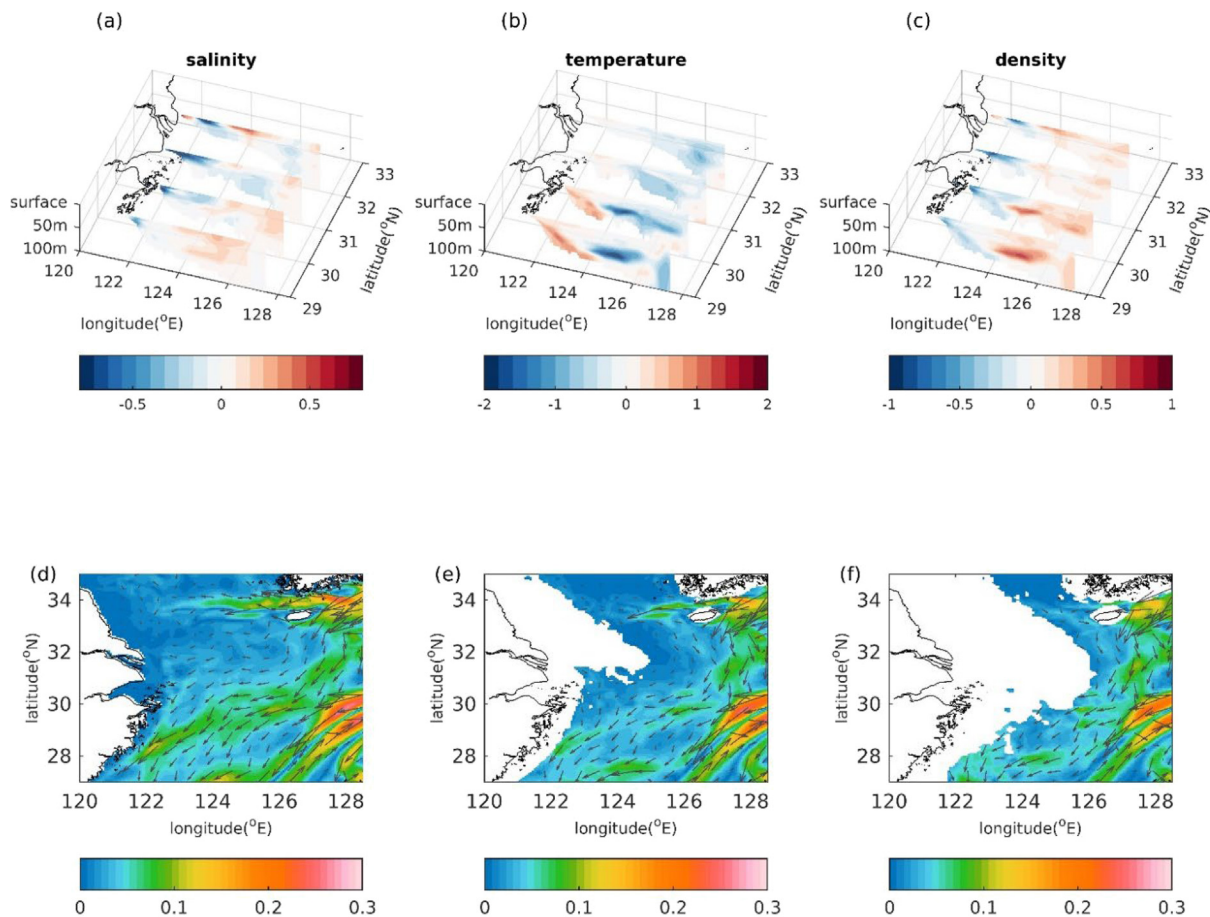
Fig. 15. The composites of Type II (a) salinity (b) temperature (c) density anomaly during July. (d)–(f) anomalous circulation (m/s) at 10 m, 40 m, and 70 m during July, respectively.
