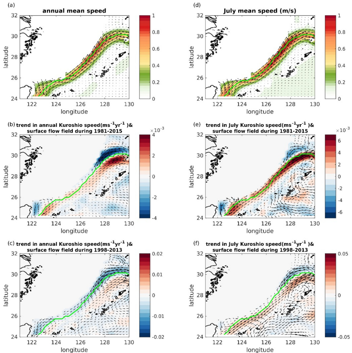
Fig. 7. (a) Annual Kuroshio mean speed ( <200 m, m/s), and linear trend in annual Kuroshio speed ( \text{ms}^{-1}\text{yr}^{-1} ) and flow field (b) during 1981–2015 and (c) during 1998–2013 (the global warming hiatus). The green lines shows the Kuroshio main stream (defined by the max current speed). (d)–(f) are the same as (a)–(c) except for July.
